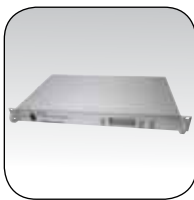
ZT-101 Switched signal leveler Ultra Reliable 1 to 15 GHz 1 x 2 matrix Gain 26+/-1 dB P OUT to 18 dBm
